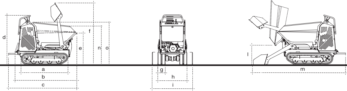
DIMENSIONS (mm)
